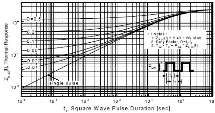
Figure 11-2. Transient Thermal Response Curve for OSF12N65C
