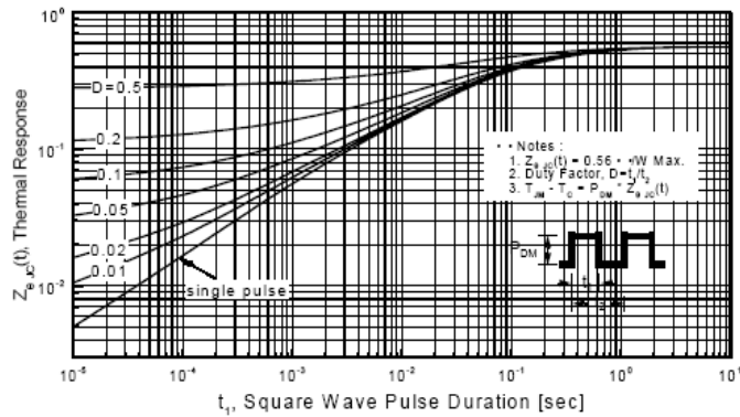
Figure 11-1. Transient Thermal Response Curve for OSP12N65C
