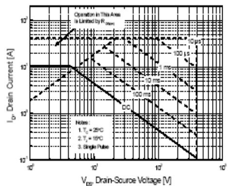
Figure 9-2. Maximum Safe Operating Area for OSF740C
